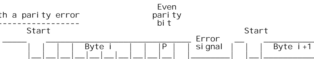
Figure 8 : Byte transmission diagram -----
