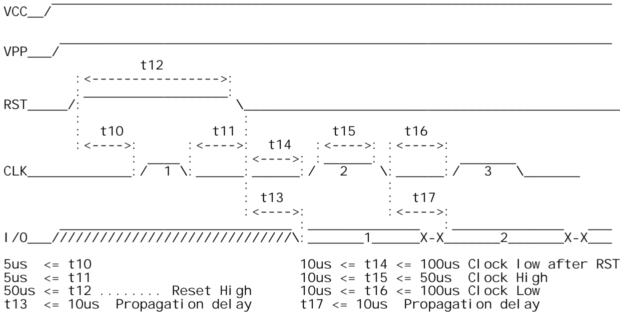
Figure2 : Reset of the card when a synchronous answer is expected.
