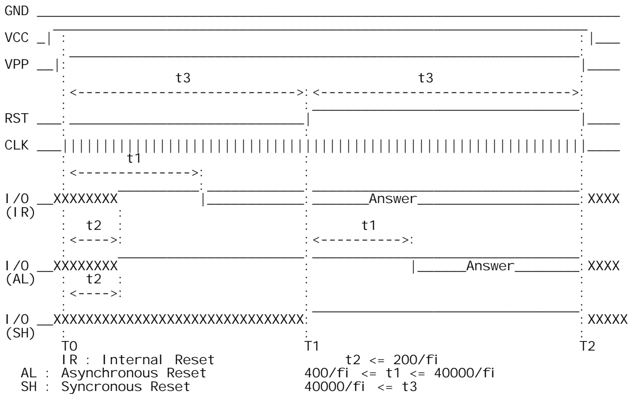
Figure1 : Reset of the card
